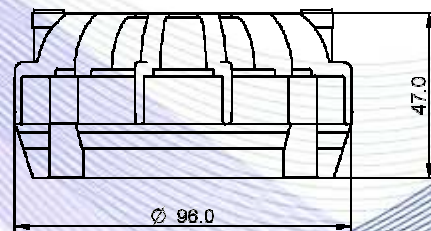
Mounting holes: 2 holes M5 on Ø70mm
